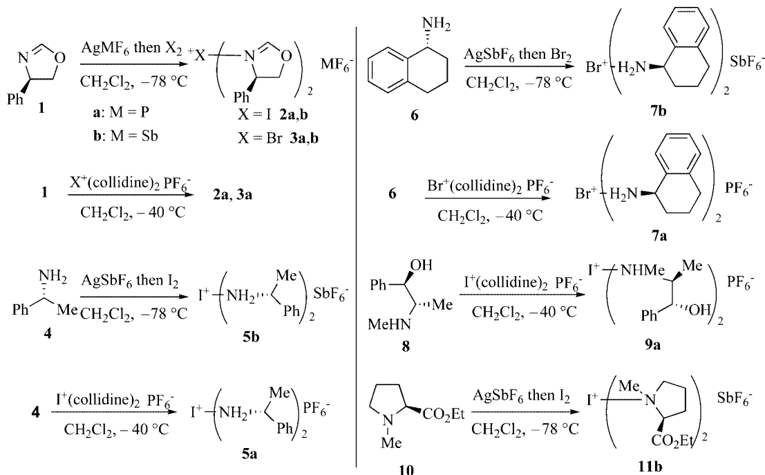
Scheme 1. Preparation of halo-bis(amine) salts.
