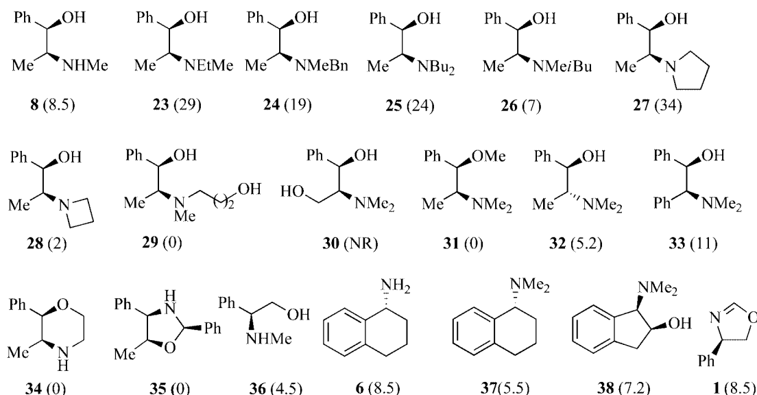
Scheme 6. ee values (%) measured for iodolactones 18 of (4 R ,5 S ) absolute configuration obtained by the iodolactonization of acid 17 with various amines.
