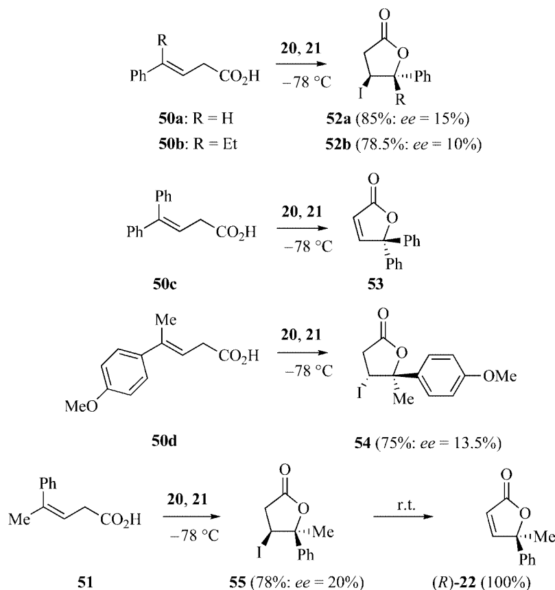
Scheme 11. Iodolactonization of acids 50a–d and 51 .
