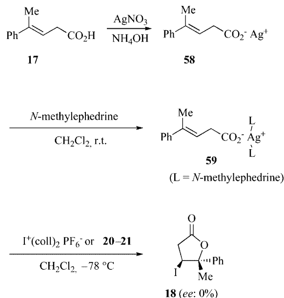
Scheme 13. Preparation and iodolactonization of the silver complex 59 .
