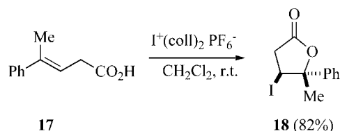
Scheme 3. Iodolactonization of acid 17 .
