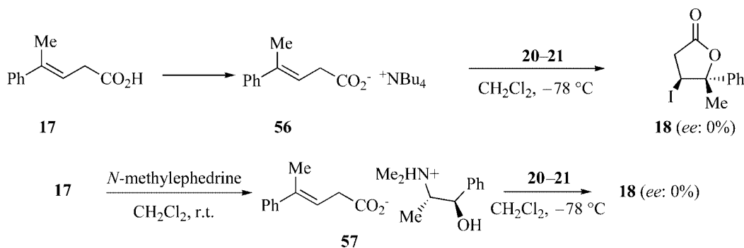
Scheme 12. Iodolactonization of salts 56 and 57 .
