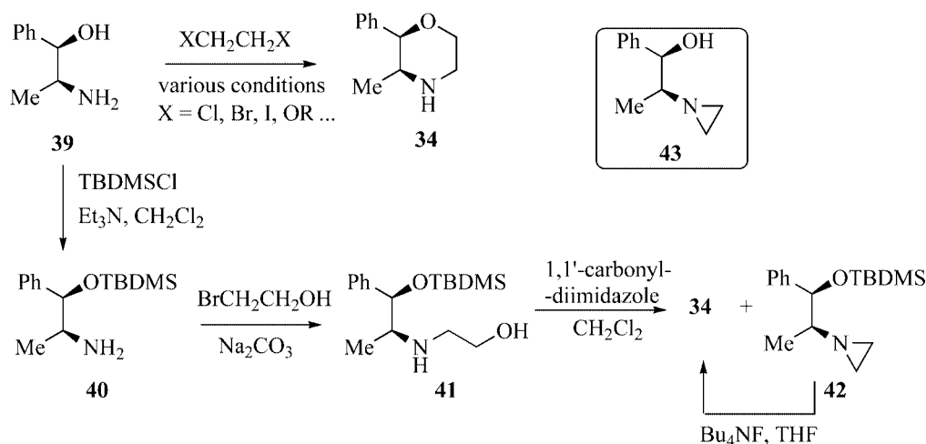
Scheme 7. Attempts at the preparation of aziridine compound 43 .
