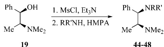
Scheme 8. Preparation of diamines 44–48 .
