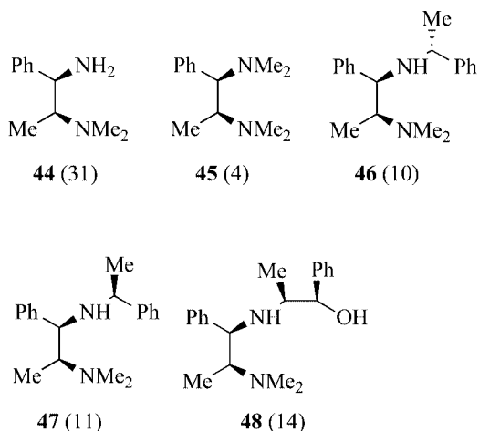
Scheme 9. ee values (%) measured for iodolactones 18 of (4 S ,5 R ) absolute configuration obtained by the iodolactonization of acid 17 with diamines 44–48 .
