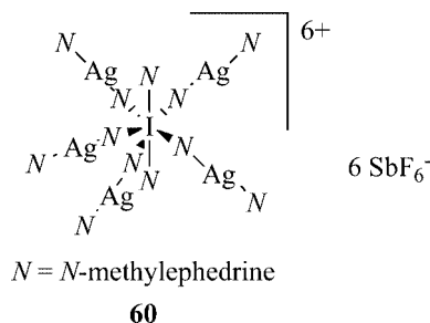
Scheme 14. Postulated structure of complex 60 .
