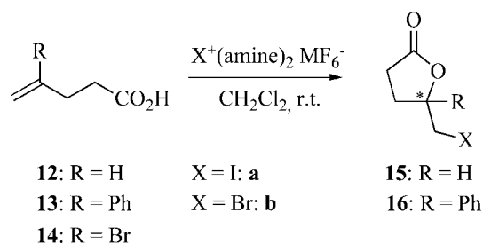
Scheme 2. Preparation of halo-lactones 15 and 16 .
