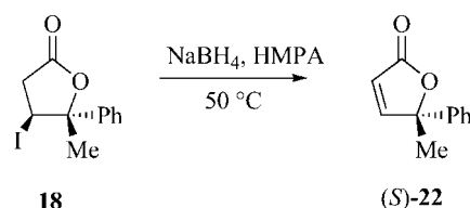
Scheme 5. Preparation of lactone 22 .
