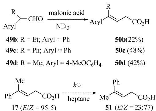
Scheme 10. Preparation of 4-arylbut-3-enoic acids 50b–d and 51 .
