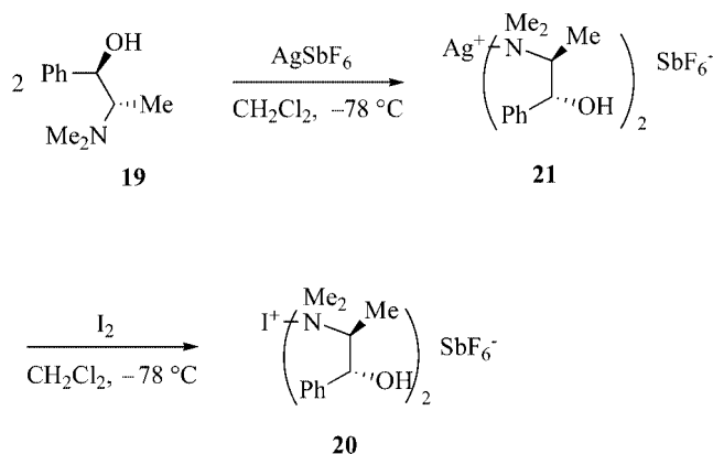
Scheme 4. Preparation of complexes 20 and 21 .
