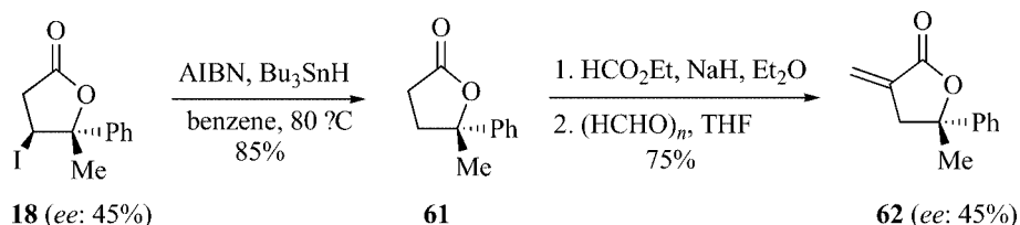
Scheme 15. Preparation of lactone 62 .
